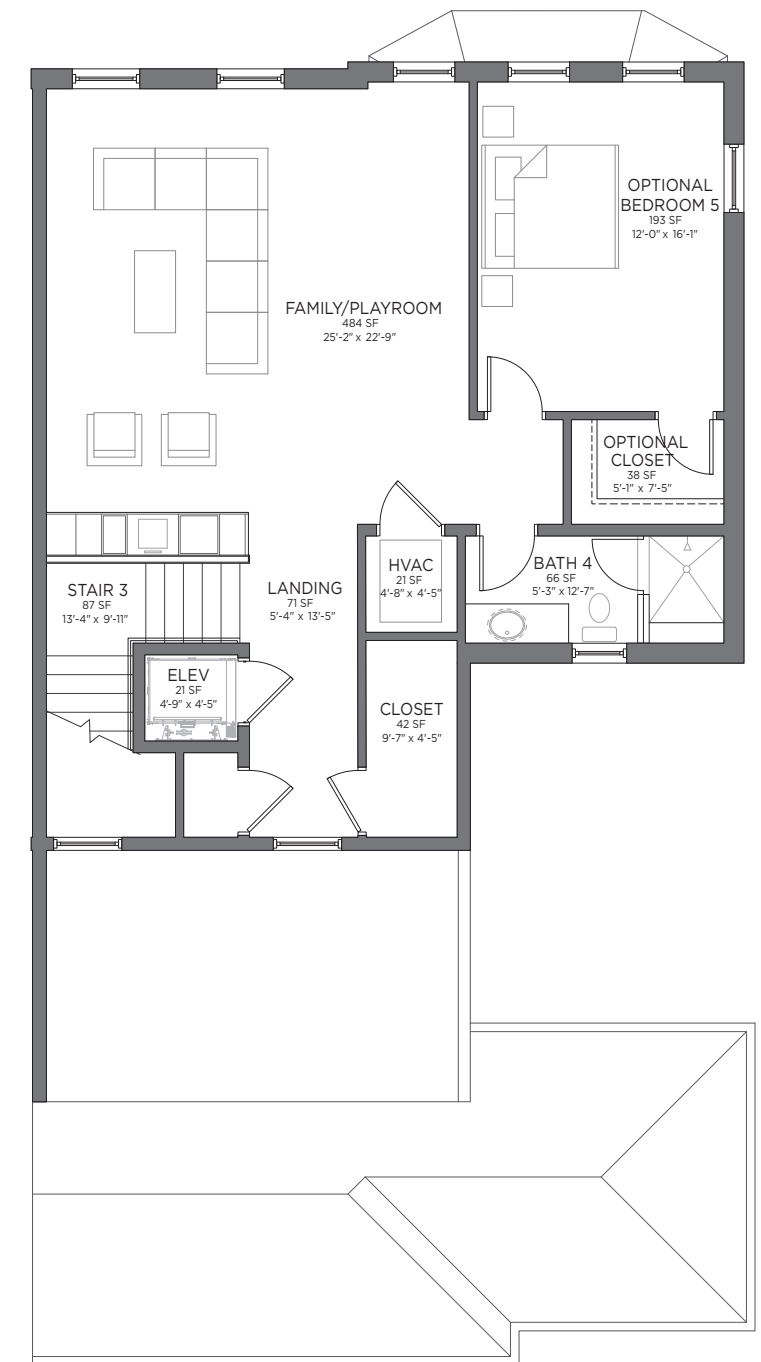
3rd Floor (Optional Bedroom 5)
